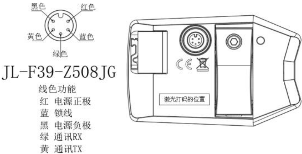
Pinout table
